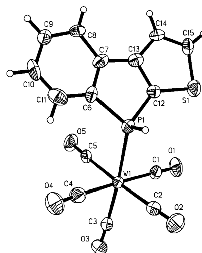
Figure 1. X-ray crystal structure of 4f . Main bond lengths (Å) and angles (°): P1–W1 2.4845(14), P1–C6 1.817(5), P1–C12 1.811(5), C6–C7 1.380(7), C12–C13 1.384(6), C7–C13 1.456(7), C12–S1 1.743(5), S1–C15 1.710(11), C13–C14 1.479(11), C14–C15 1.343(11); C6–P1–C12 89.4(2), C12–S1–C15 93.0(4).
